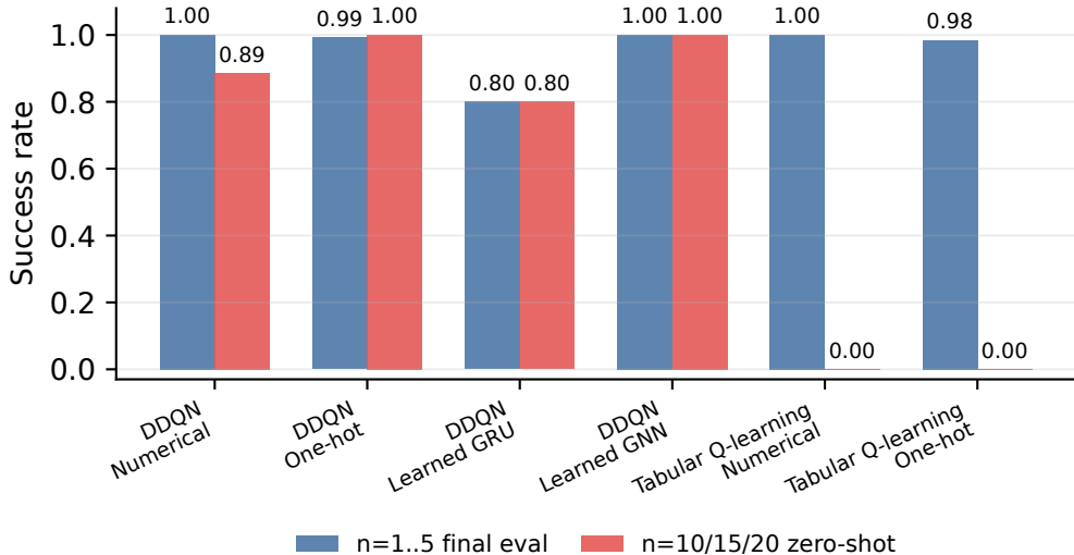
In-distribution vs zero-shot success
