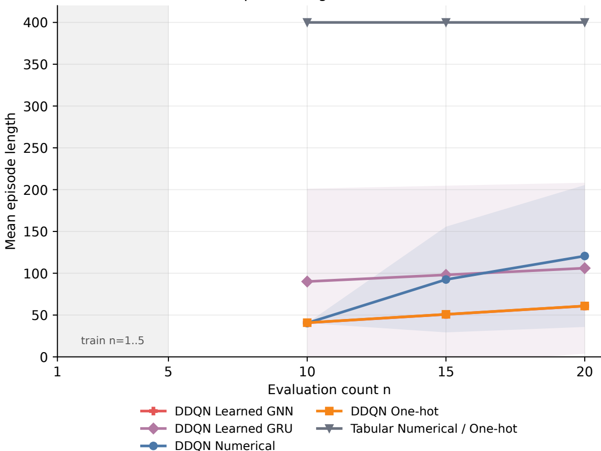
Zero-shot episode length with tabular contrast
