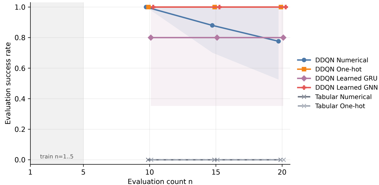
Zero-shot generalization with tabular contrast
