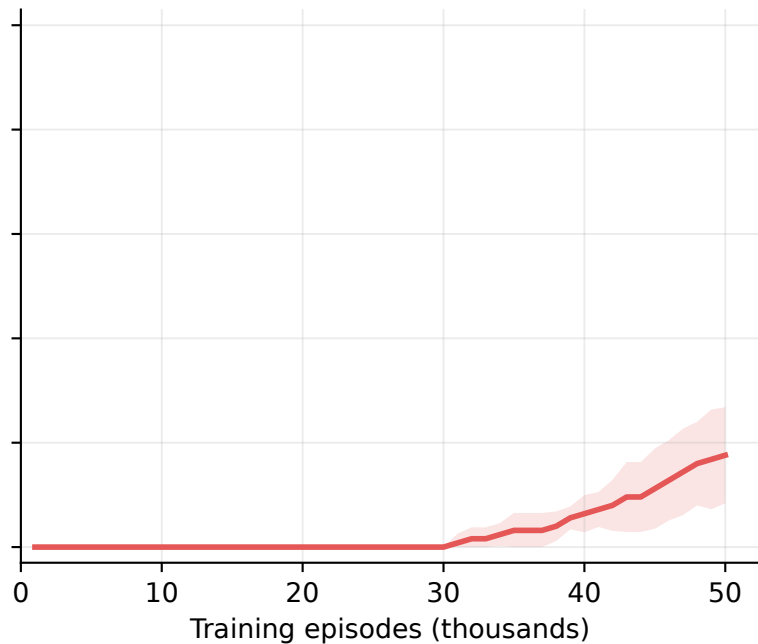
Q-learning
