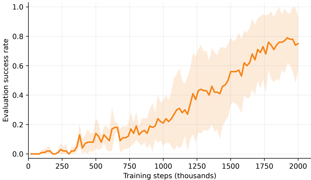
Full-random LetterEnv learning curve
