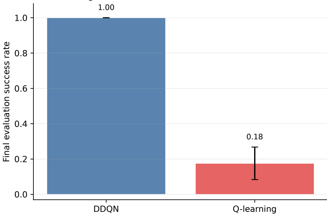
Regional randomized LetterEnv: final success
