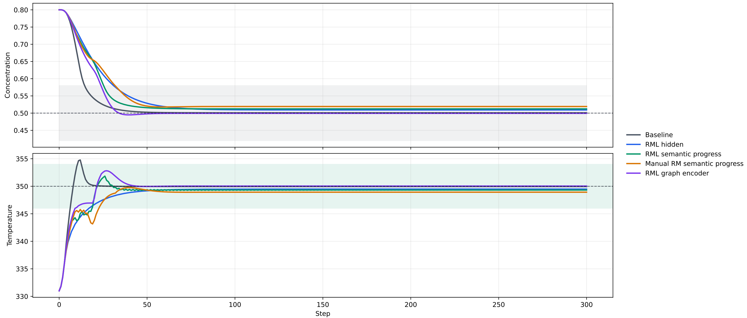
CSTR trajectory comparison, seed 0 with RML hidden seed 2 and manual RM seed 1
