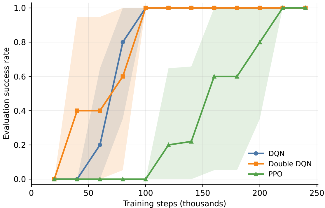
Learning curves by algorithm
