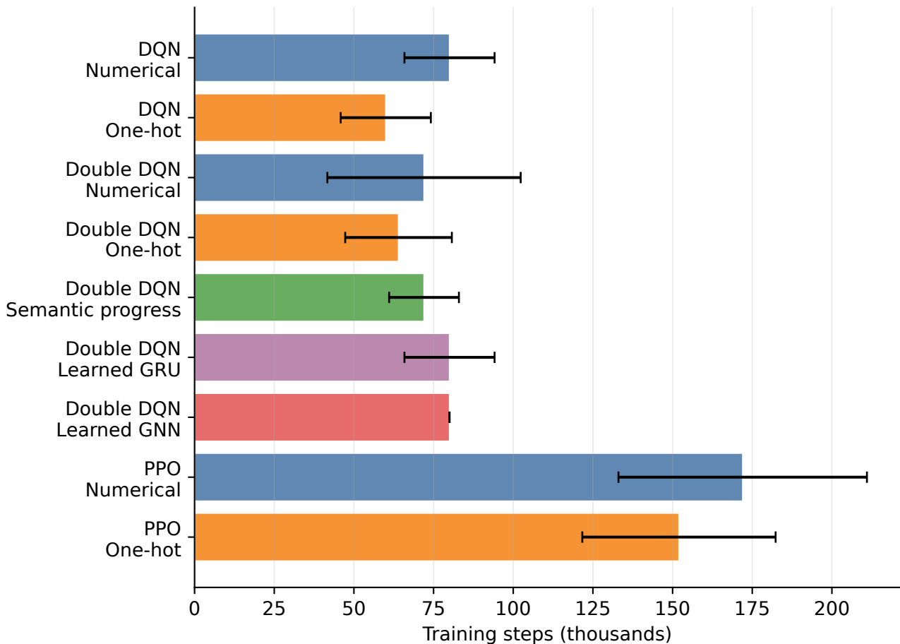
Sample efficiency to success rate \geq 0.9
