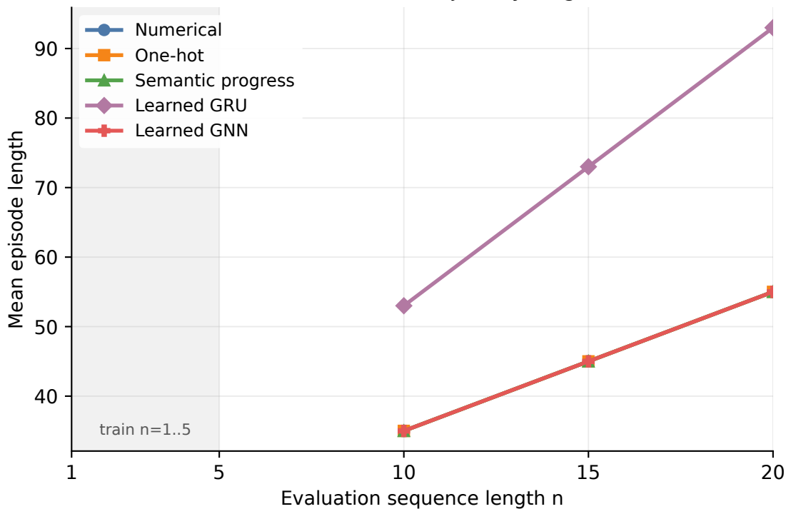
DDQN zero-shot trajectory length
