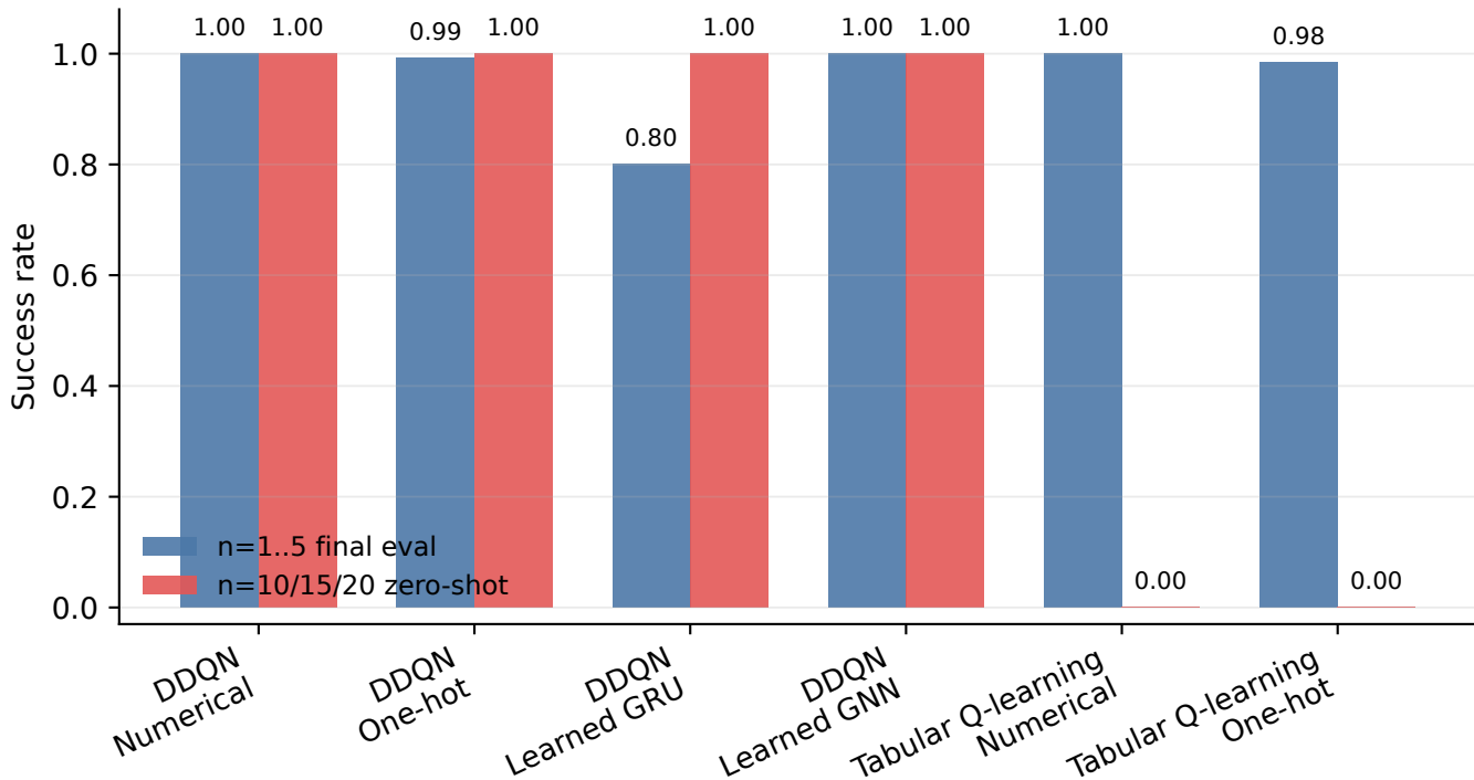
In-distribution success and zero-shot transfer
