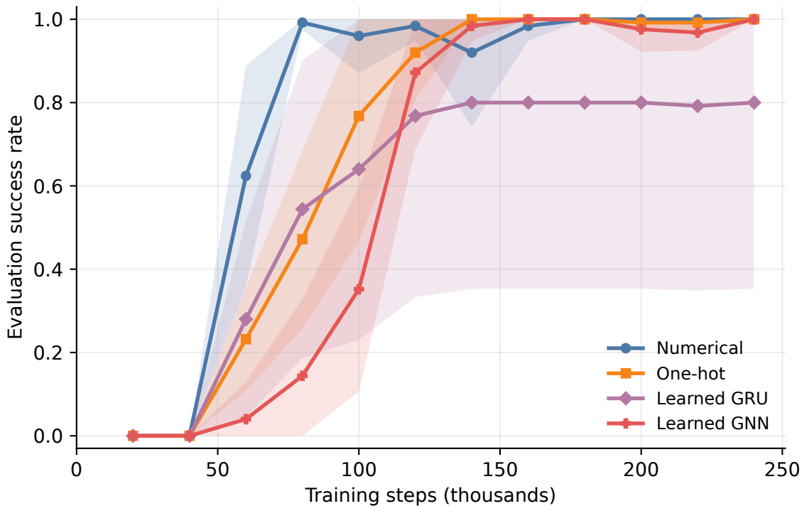
DDQN learning curves by encoding
