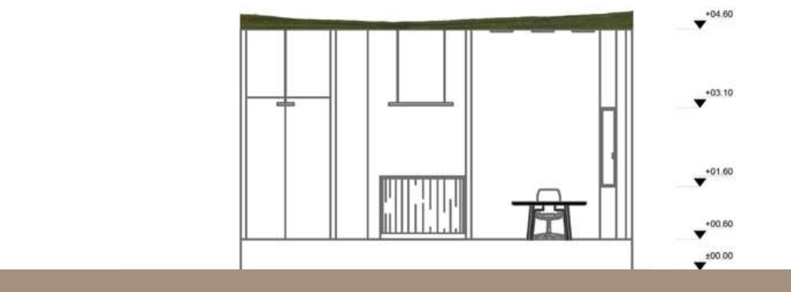
A-A SECTION CUT SCALE : 1/100
