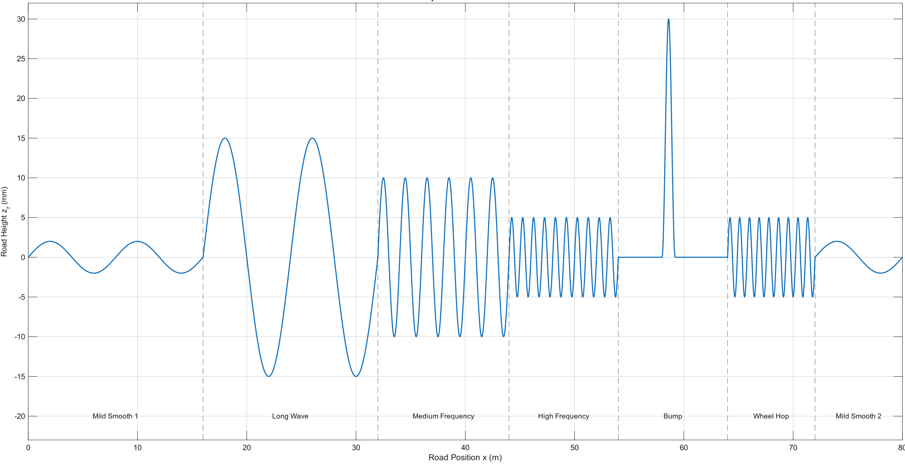
Common Composite Benchmark Road Profile
