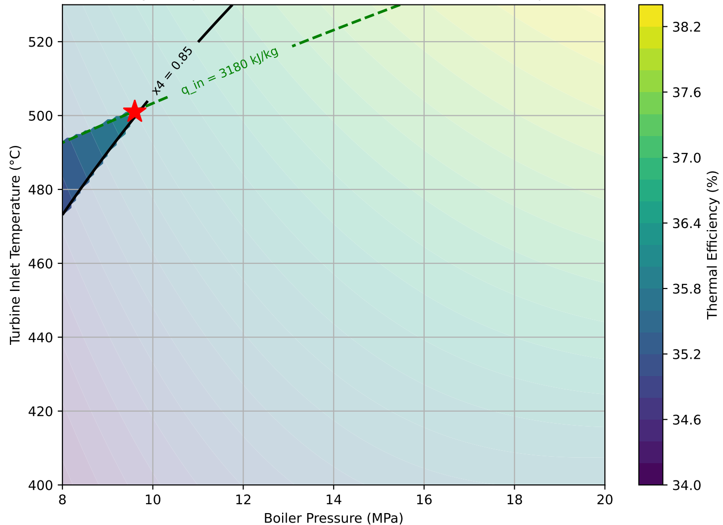
Rankine Cycle Optimization - Boiler Pressure vs Turbine Temperature
