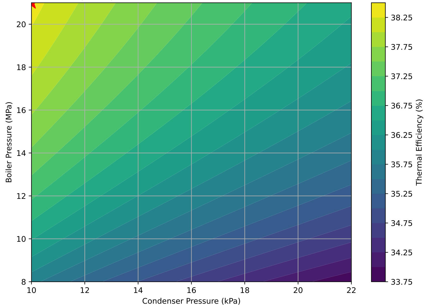
Rankine Cycle Optimization - Condenser Pressure vs Boiler Pressure
