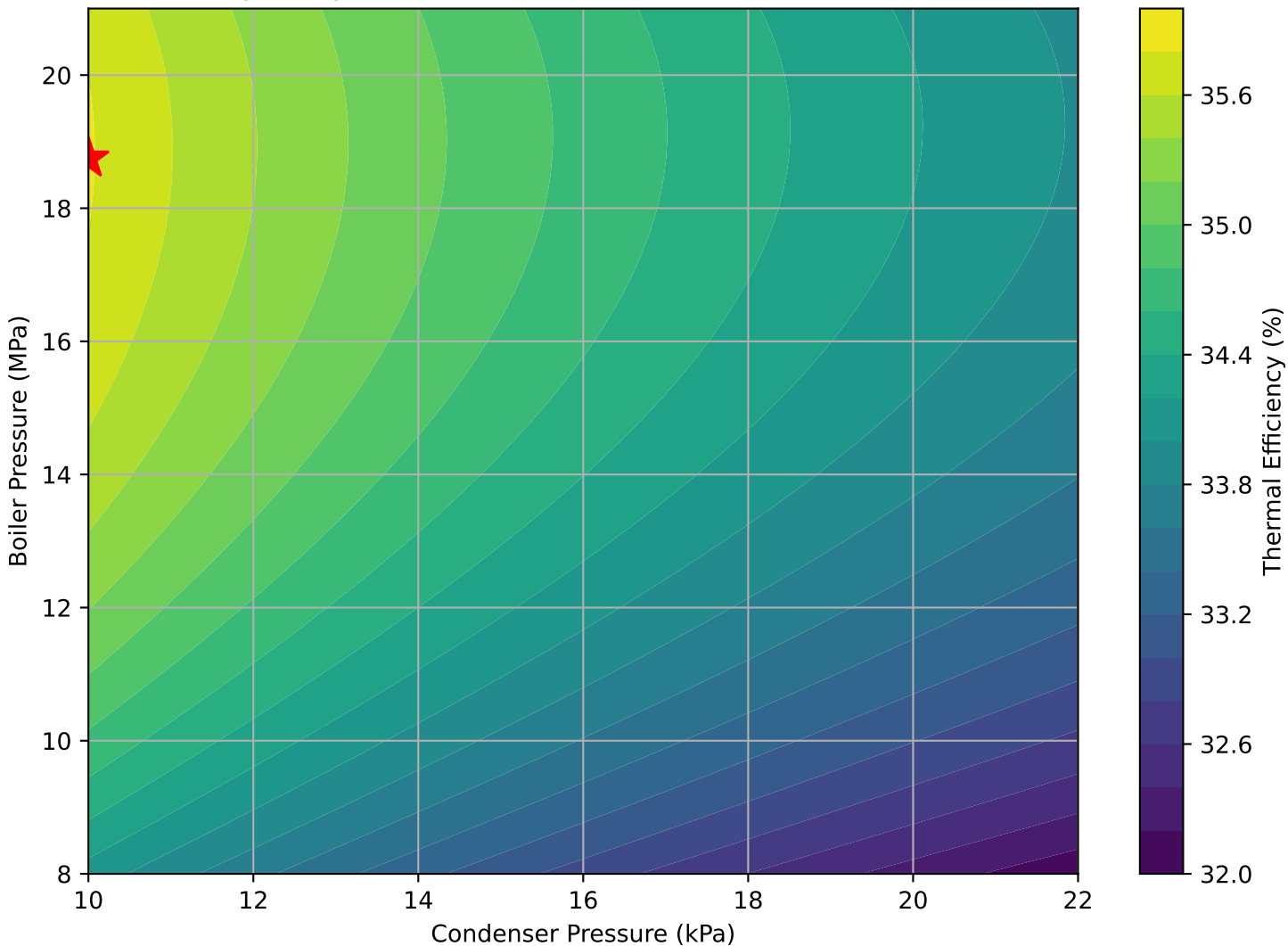
Rankine Cycle Optimization - Condenser Pressure vs Boiler Pressure
