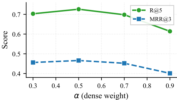
Convex Combination: Effect of \alpha
