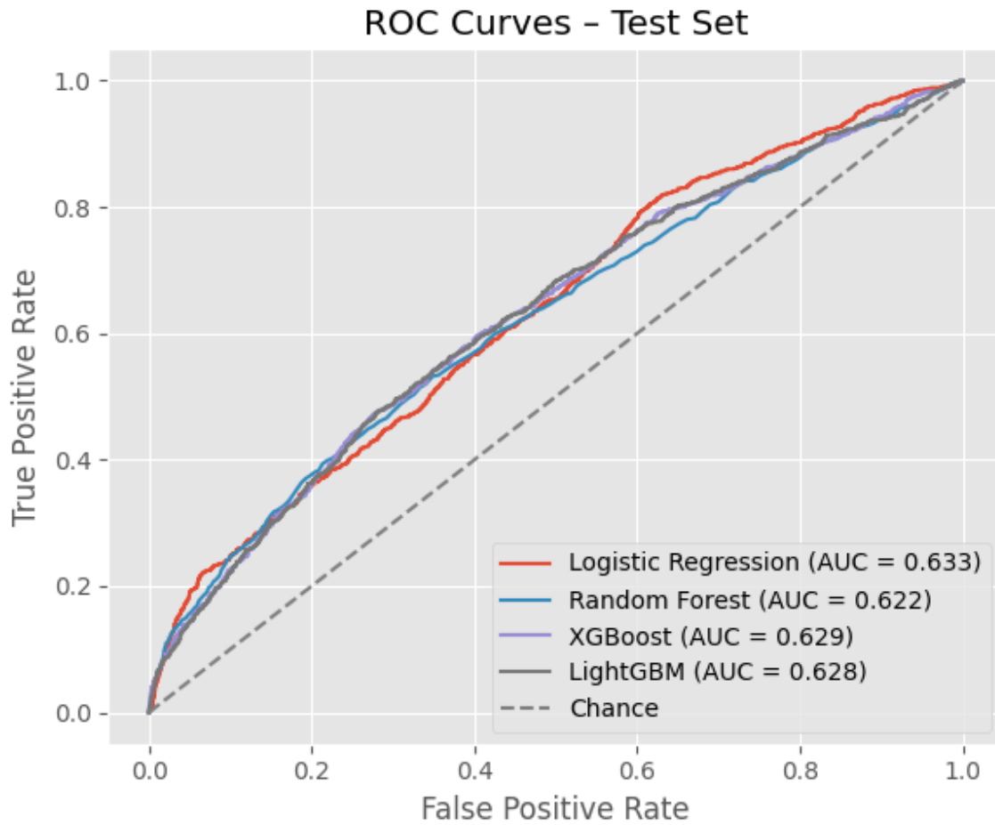
Figure 4. ROC curve figure saved in 03_modeling.ipynb output.
