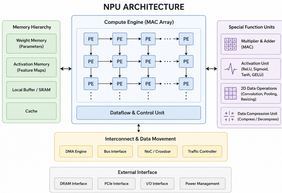
Figure 1: Simplified NPU Architecture
