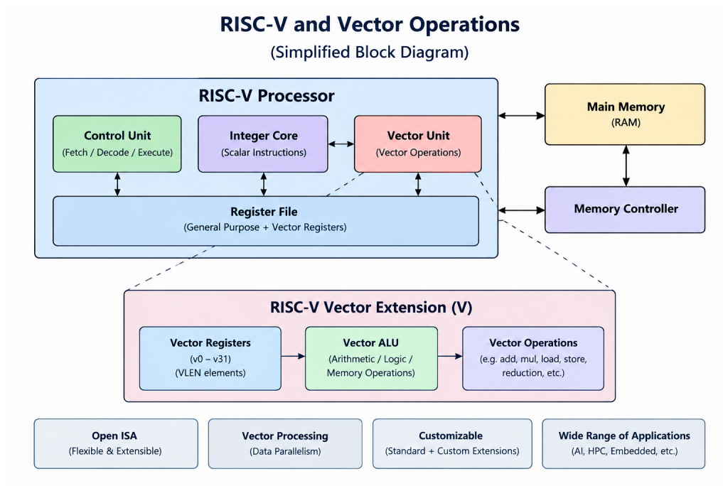
Figure 3: RISC-V Vector Operations Block Diagram
