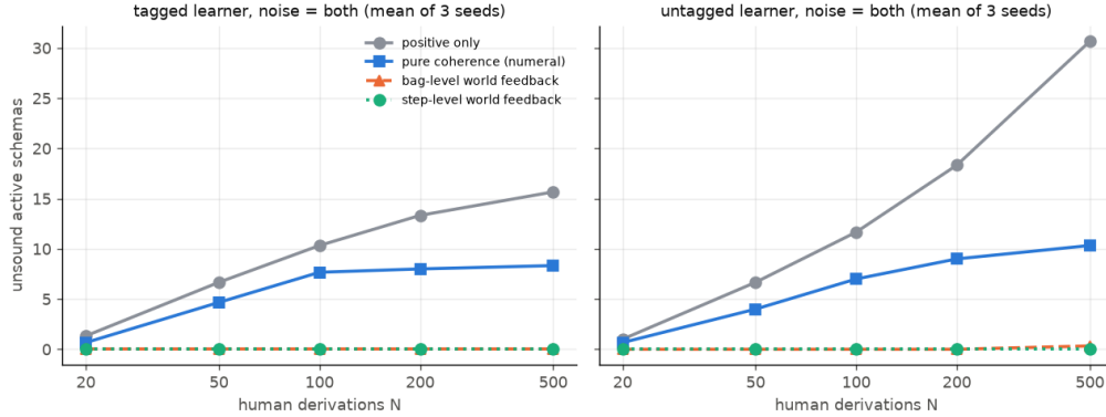
Figure 1: Experiment A: unsound active schemas against the number of human derivations N (noise both , mean of three seeds), tagged learner (left) and untagged learner (right) (computed). Imitation alone (grey) gets worse with N ; coherence without a world (blue) removes about half; world feedback (orange, green) leaves one schema in one run.
