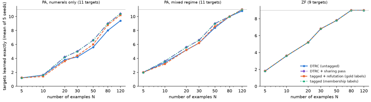
Figure 2: E5: targets learned exactly after N examples, mean over seeds 0–4 (rows of one stream share seeds). Left: PA, numerals only (11 targets); middle: PA, mixed regime; right: ZF (9 targets) experiments E5 .
