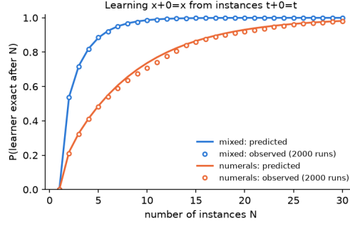
Figure 1: E1: probability that the \text{DT}_F^\circ learner is exact after N instances of x + 0 = x , observed (2000 runs) and predicted by Theorem 4.4(a) and Proposition F.8, mixed and numerals-only regimes experiments E1 .
