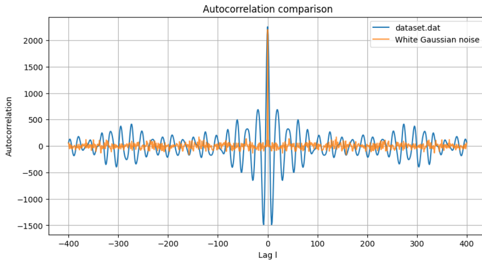
Figure 6: When comparing the autocorrelation of white noise to the dataset signal, it is clear that there is a singular place where the signal is a perfect match, so the autocorrelation of a white noise gaussian signal has a clear maximum at lag 0.
