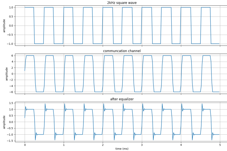
Figure 2: 2kHz testsignal, passed through, first the communication channel and then through the equalizer. Note the slight overshoot of the signal edges from the rise and fall times.
