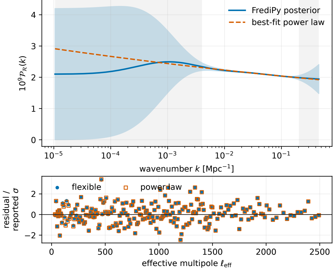
Figure 3: Conditional Planck PR3 reconstruction. The FrediPy posterior mean and its \pm 1 pointwise posterior standard deviation are compared with the best-fitting power law of equation (16); the band is not simultaneous, and grey regions lie outside the direct-sensitivity range. The lower panel shows the bandpower residuals divided by the reported diagonal errors. Their correlations are retained in the fits and in the quoted Q values.
