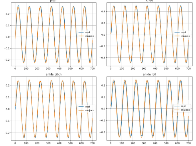
Fig. 3: Sine wave in Both MuJoCo and real-world environment. It can be found that the trajectories of the two are very close after calibration.
