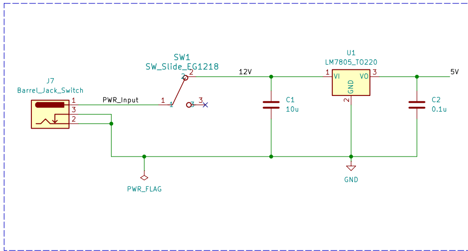
Input and 5V Circuit
