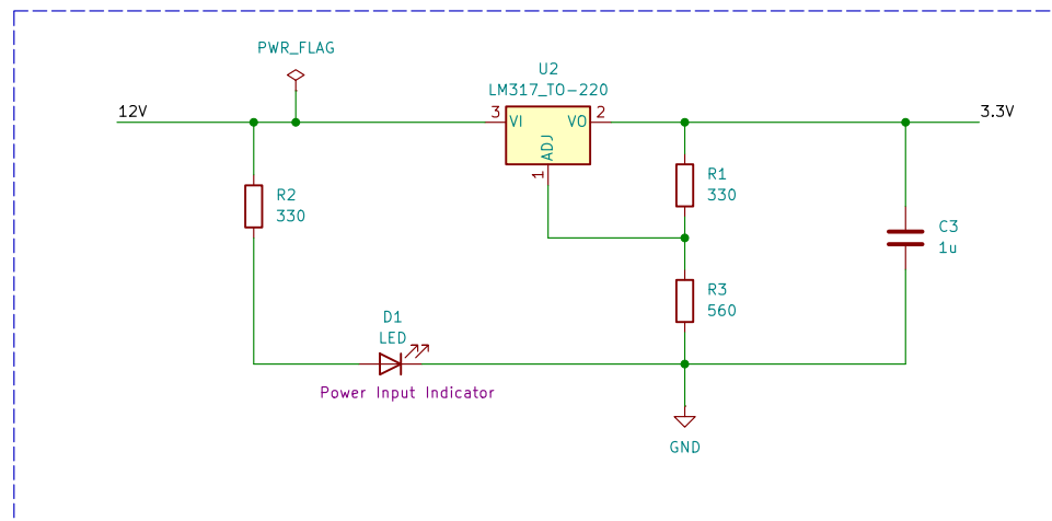
3.3V Circuit
