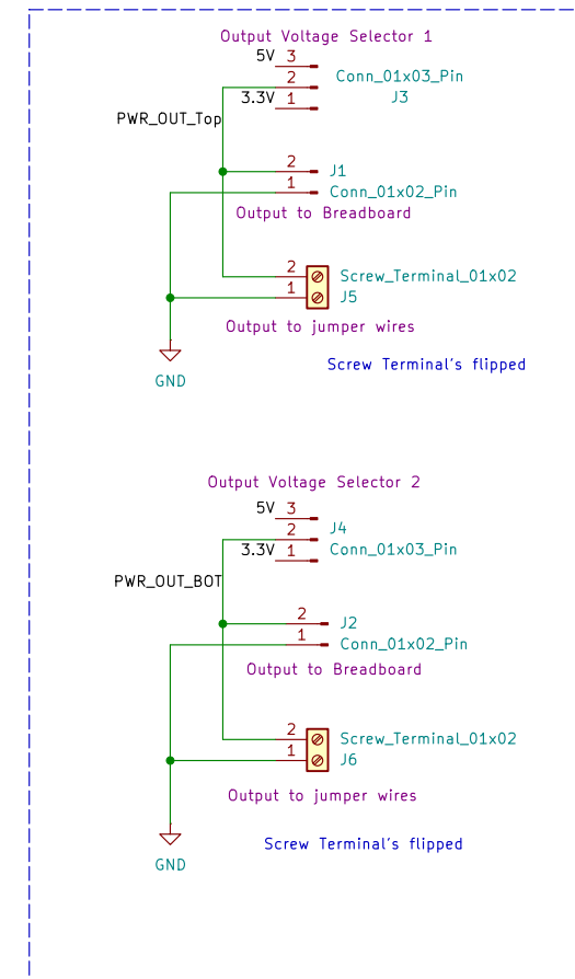
Output and Switches
