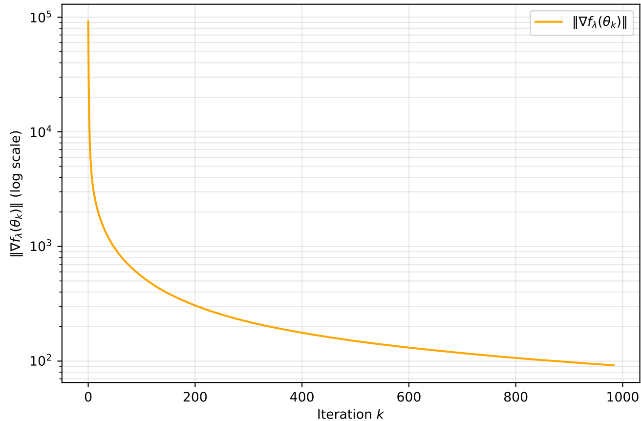
Gradient Norm vs Iteration
