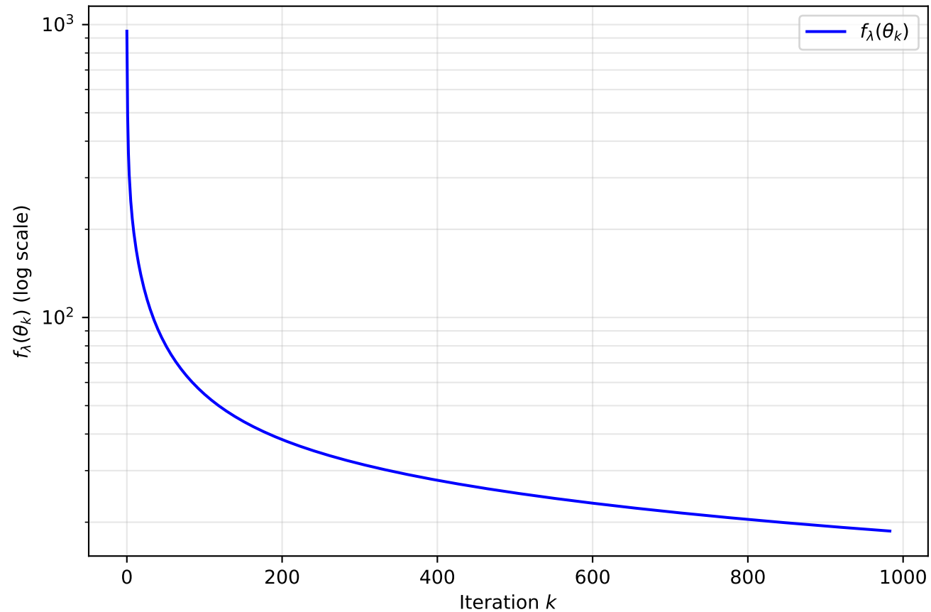
Objective Function Value vs Iteration
