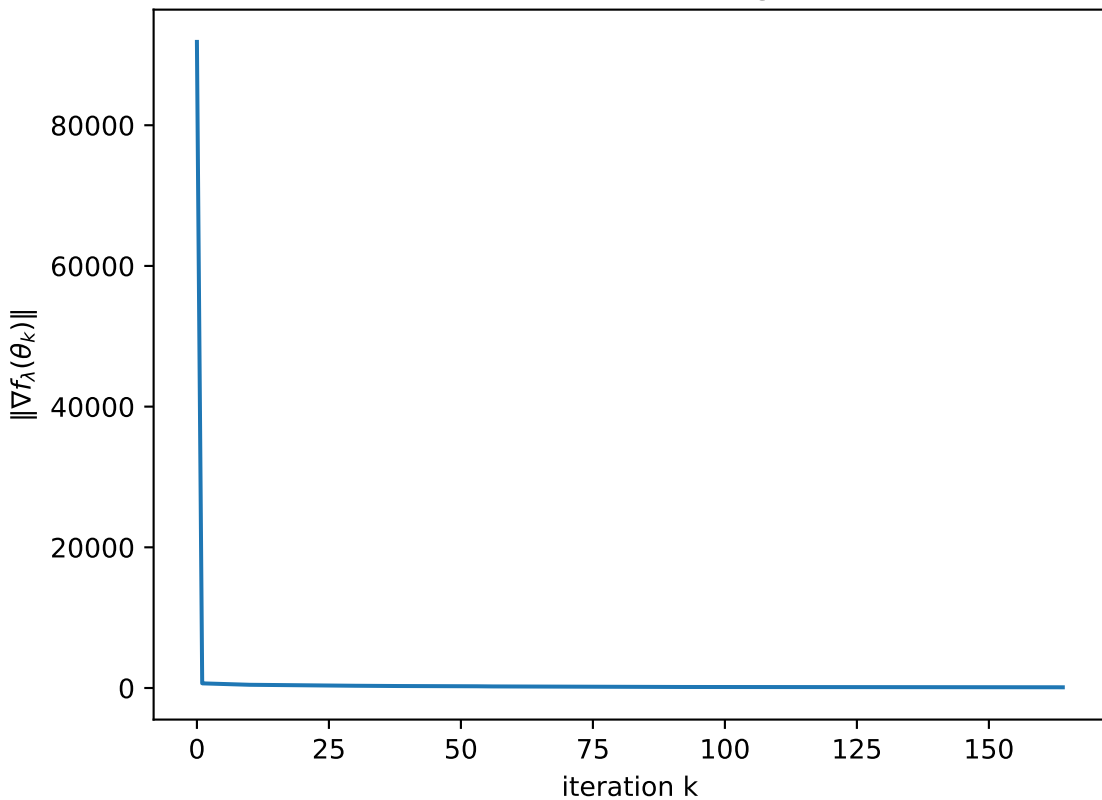
Gradient norm during GD
