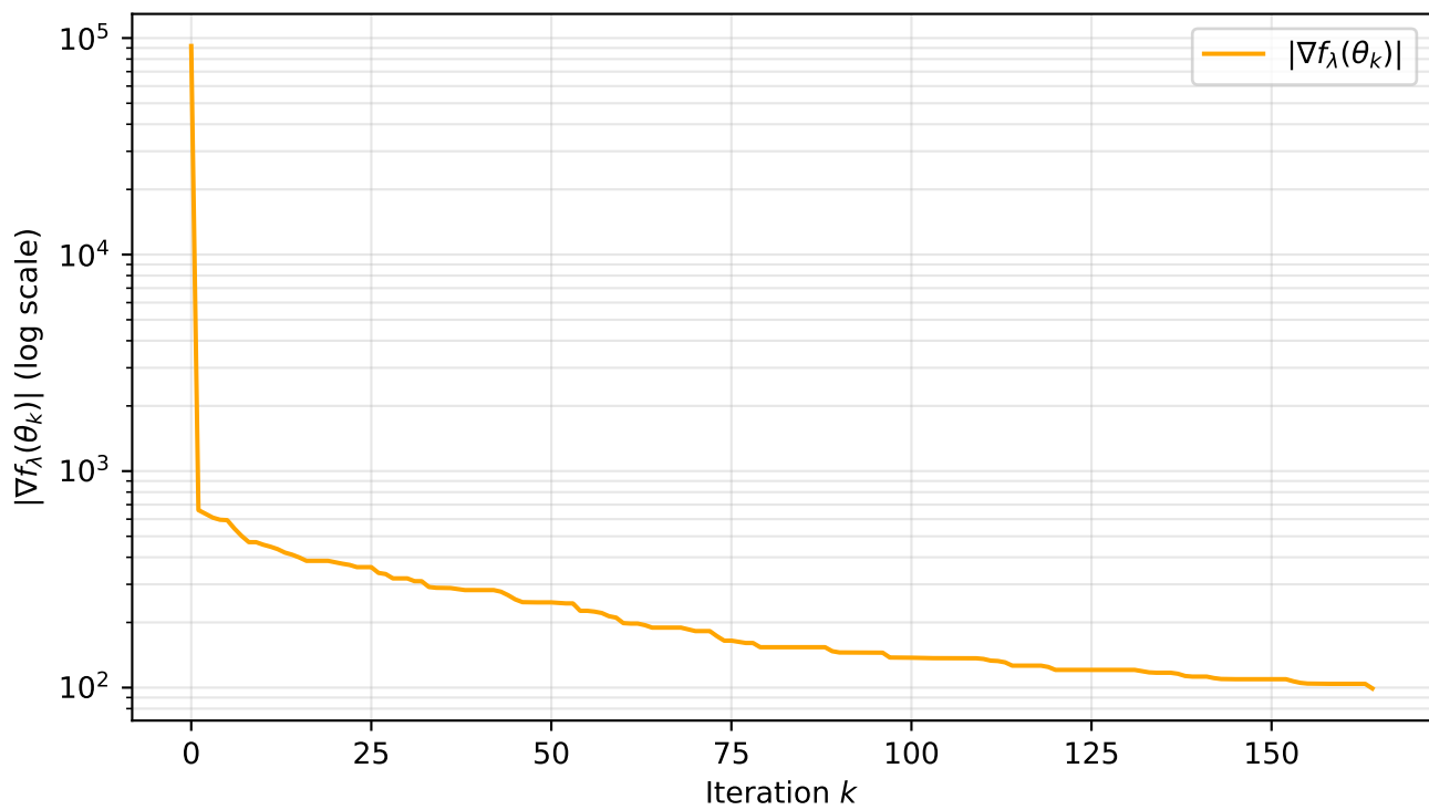
Gradient Norm vs Iteration
