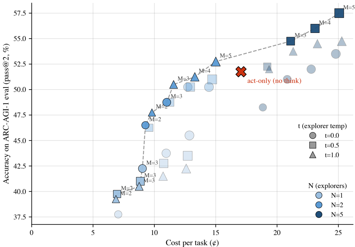
Pipeline N \times t \times M cost-accuracy surface
