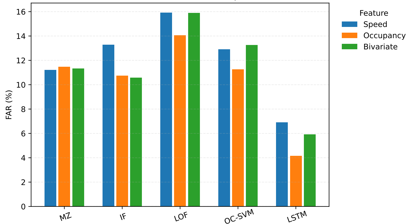
False Alarm Rate (Individual Pipeline)
