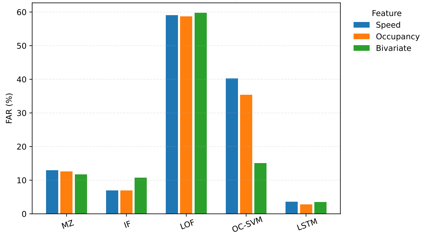
False Alarm Rate (Global Pipeline)
