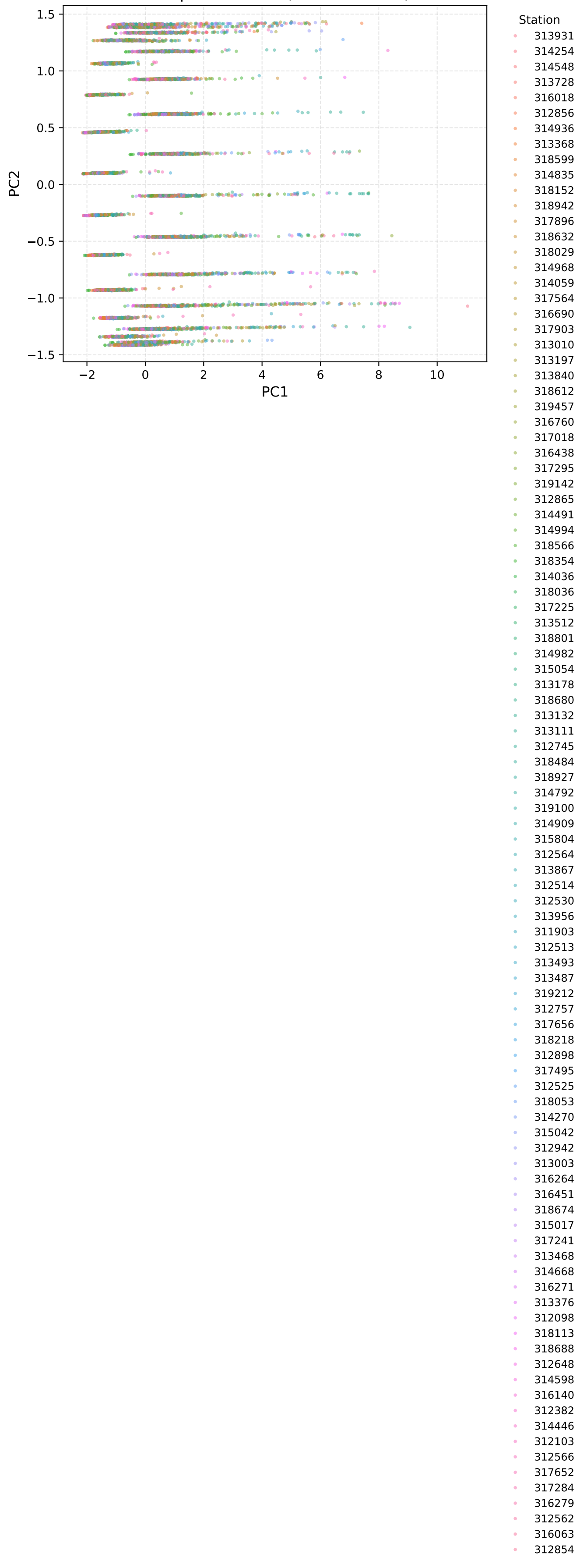
PCA: pooled TRAIN (color = station)
