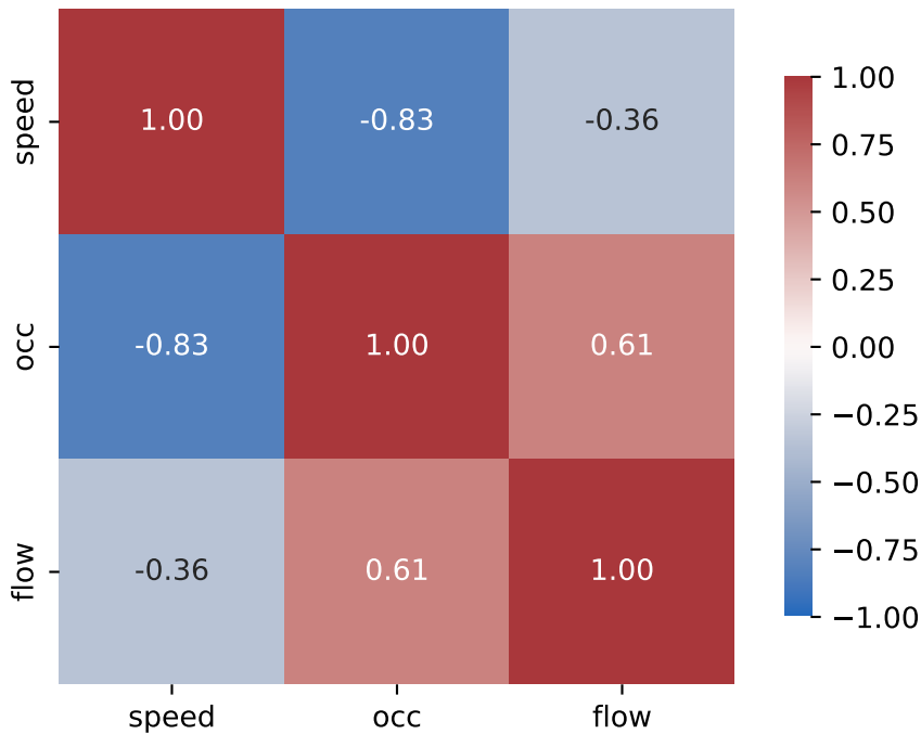
Correlation Matrix
