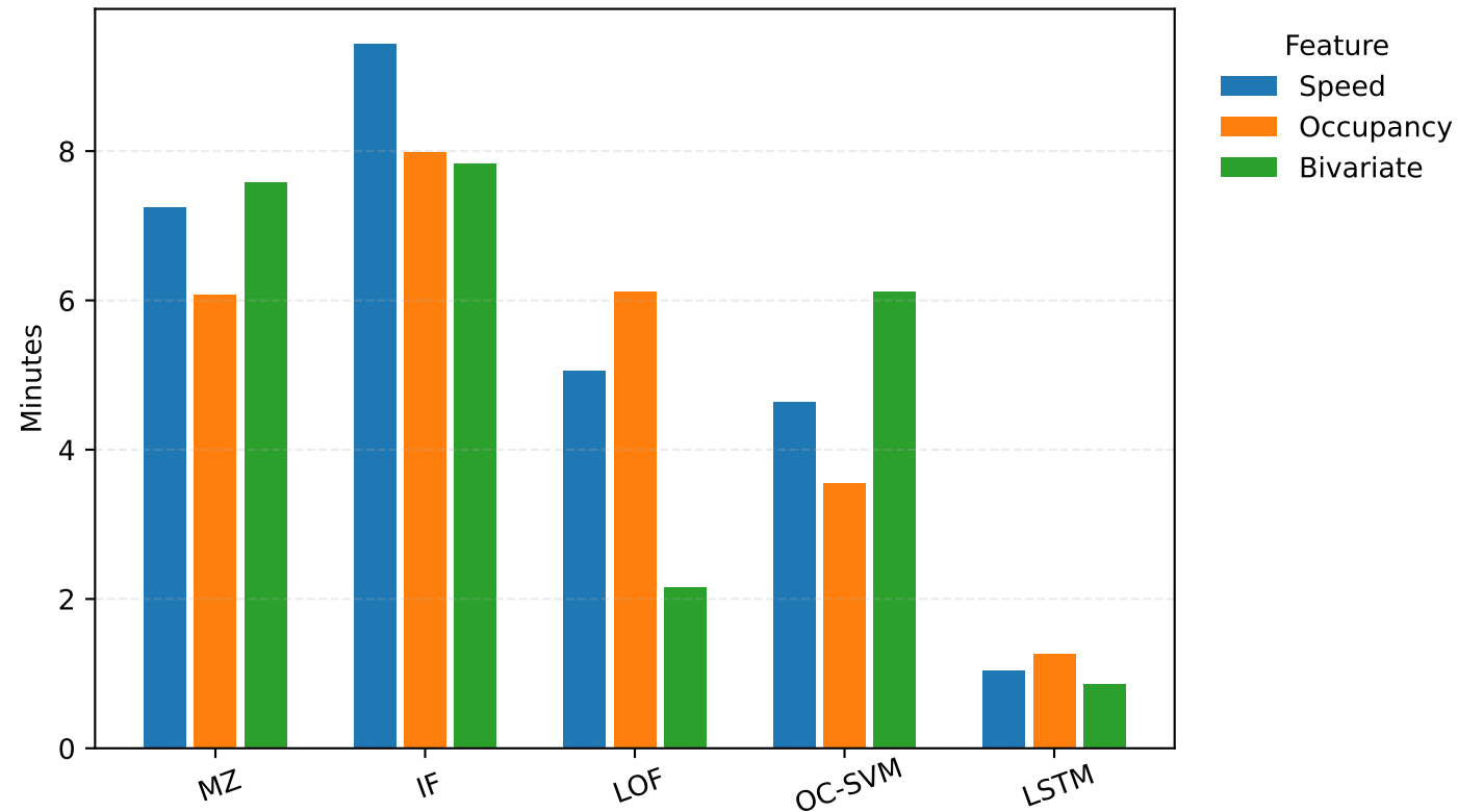
Mean Time to Detection (Global Pipeline)
