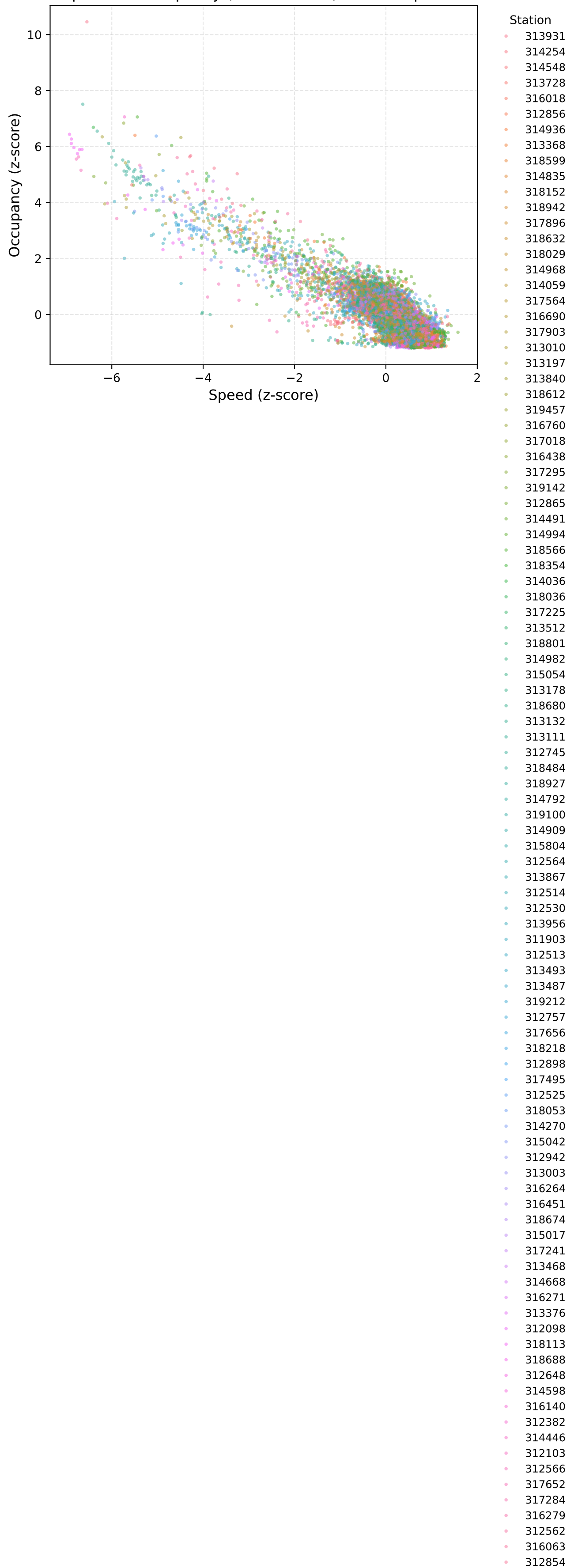
Speed vs Occupancy (standardized) — TRAIN pooled
