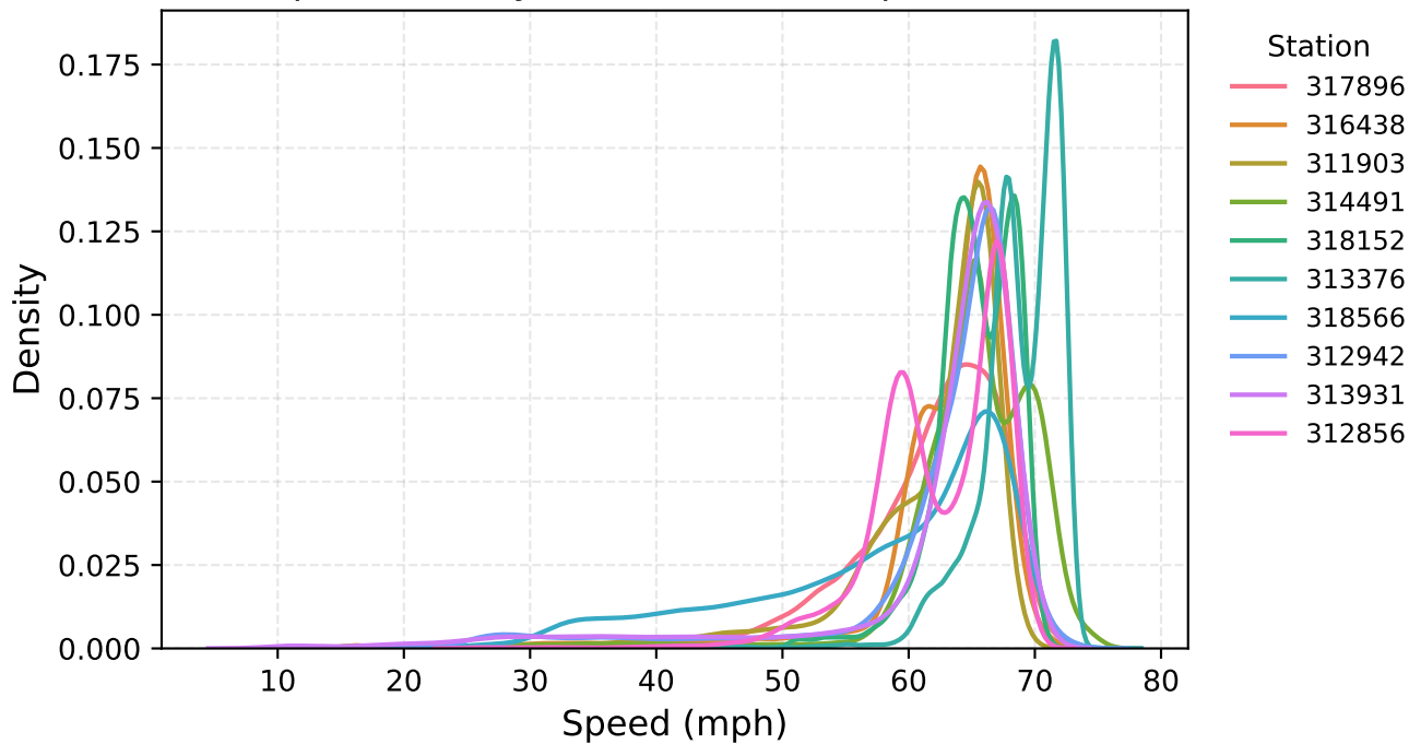
Speed KDE by station (TRAIN, top stations)
