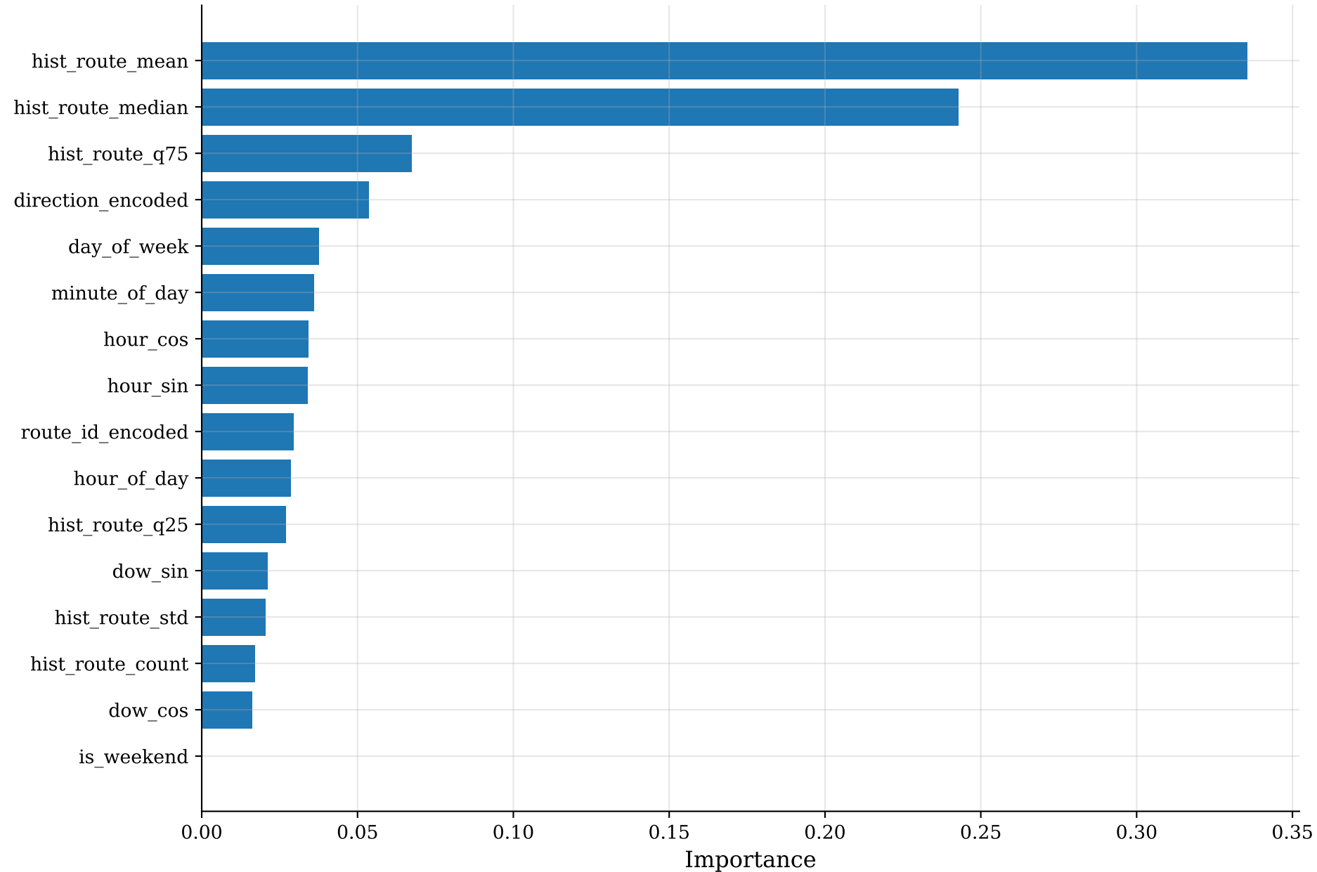
P3.3: Route-Level XGBoost Feature Importance (Top 20)
