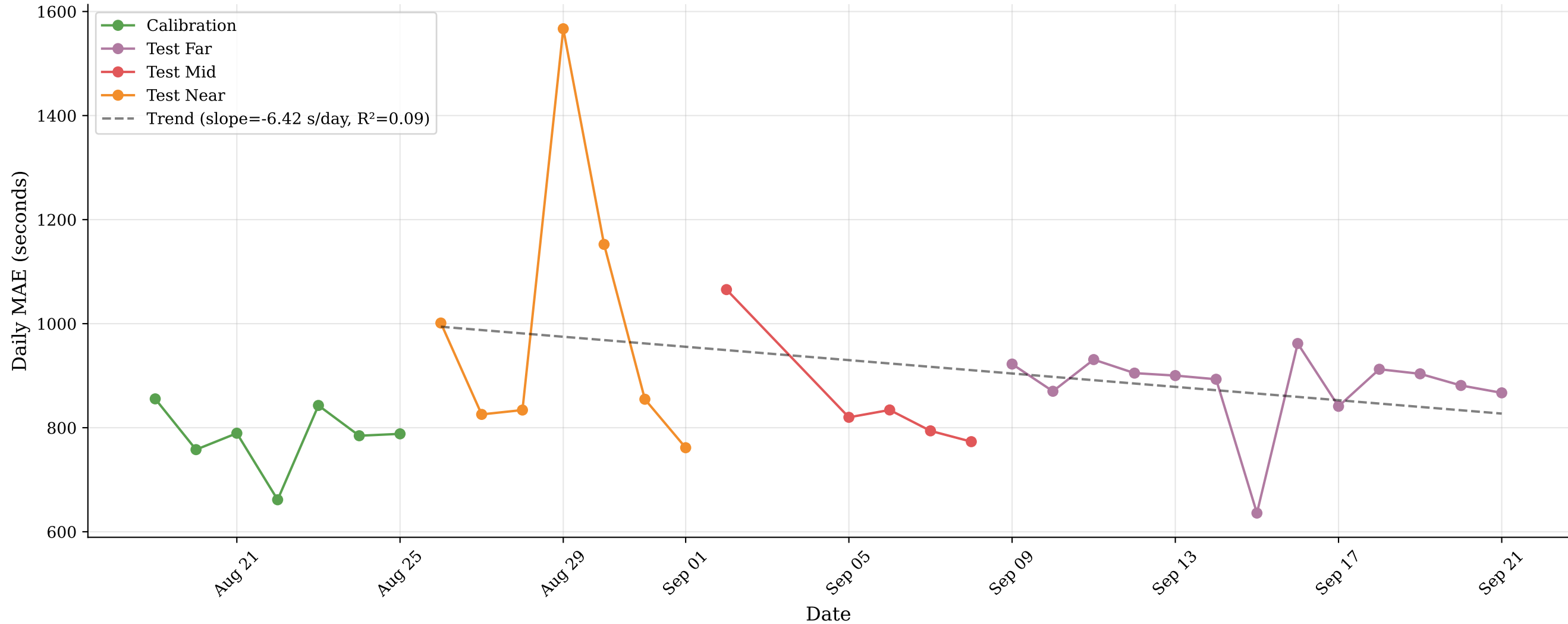
P3.5: Daily Route-Level MAE Over Test Period
