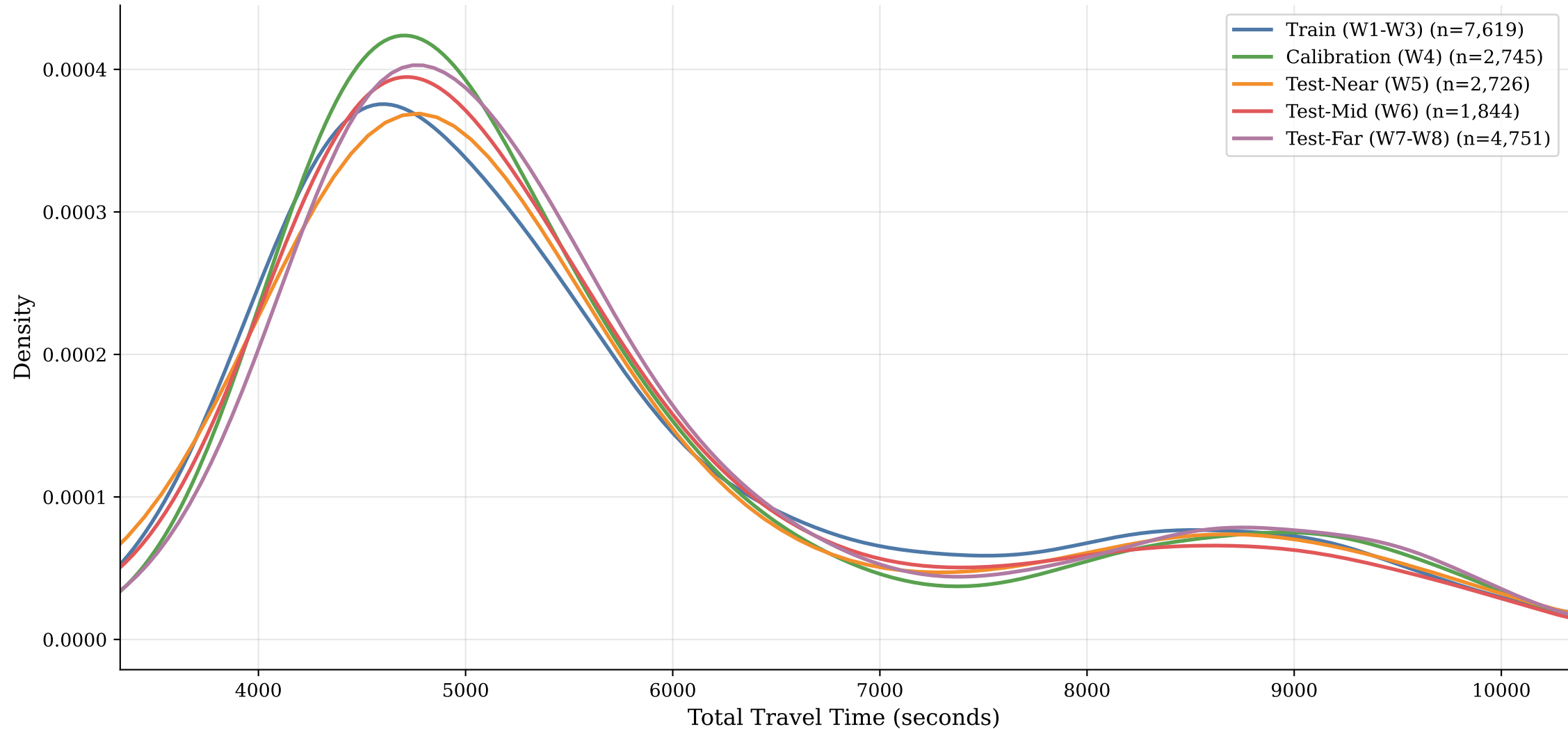
P1.5: Travel Time Distribution Comparison Across Temporal Splits
