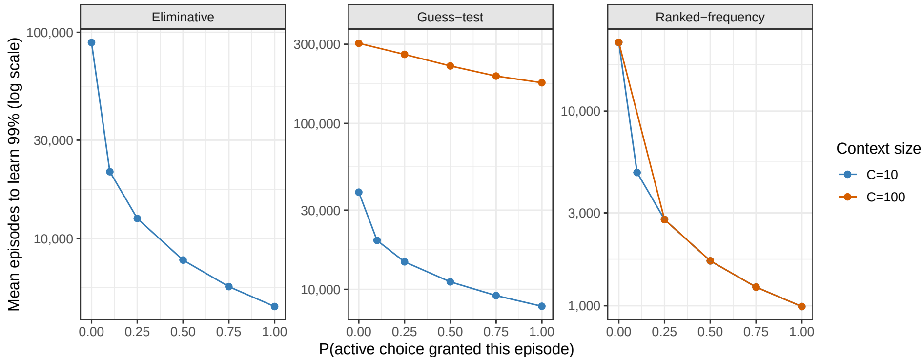
How much of the time must a learner get their choice? ( C=10 vs C=100 )
