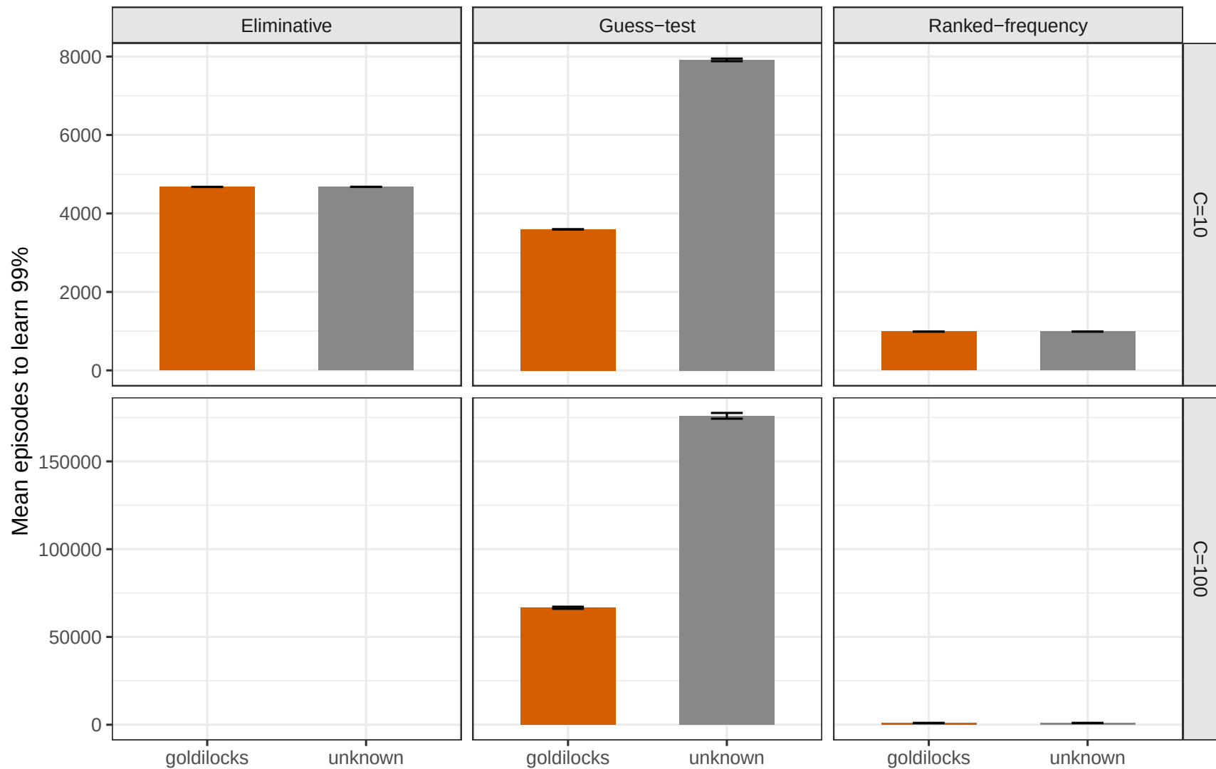
Goldilocks vs. any-unknown targeting, C=10 vs C=100
