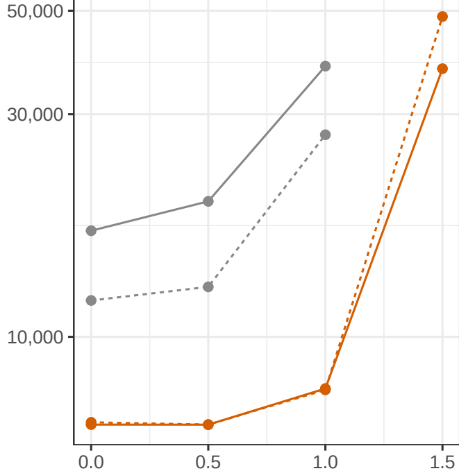
Guess-test
