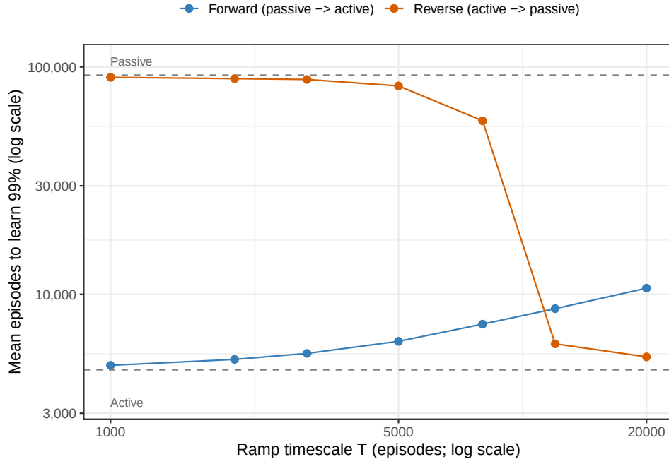
Figure G1. Mean episodes to learn 99% of the vocabulary vs. ramp timescale T , forward (passive-to-active) vs. reverse (active-to-passive) developmental trajectories. Dashed lines mark the pure passive and pure active reference points from Table G1.
