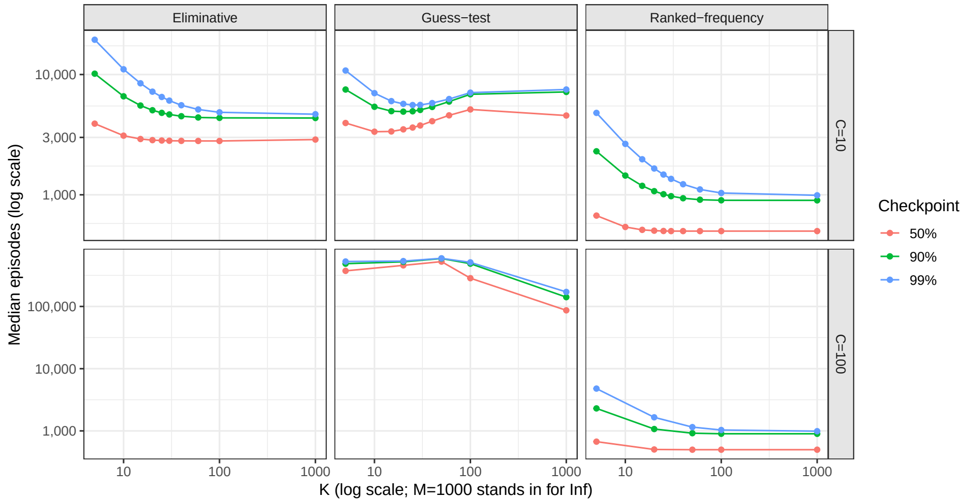
Cost of restricting the active choice set, across completion checkpoints
