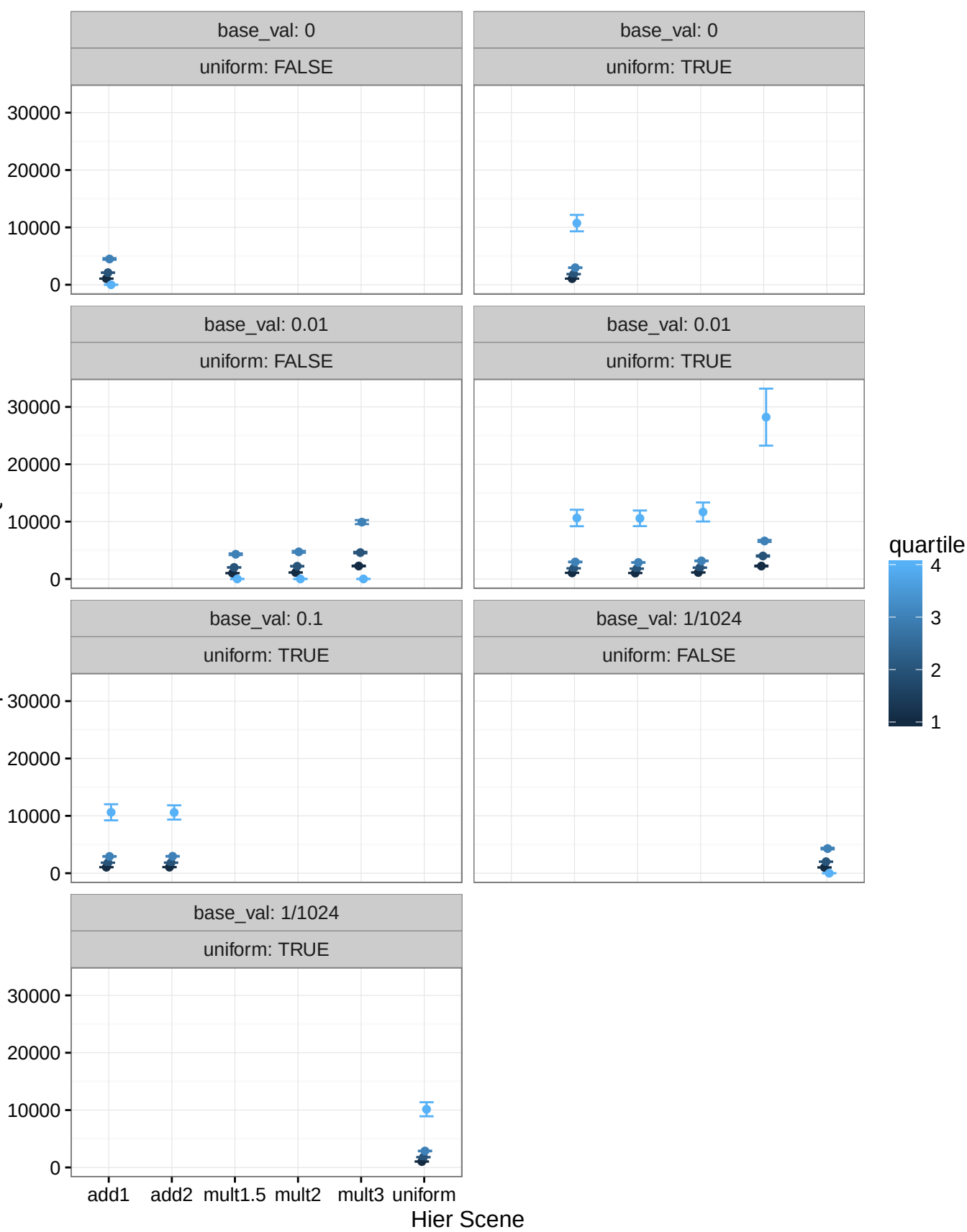
Mean # of Episodes to Reach Quartile
