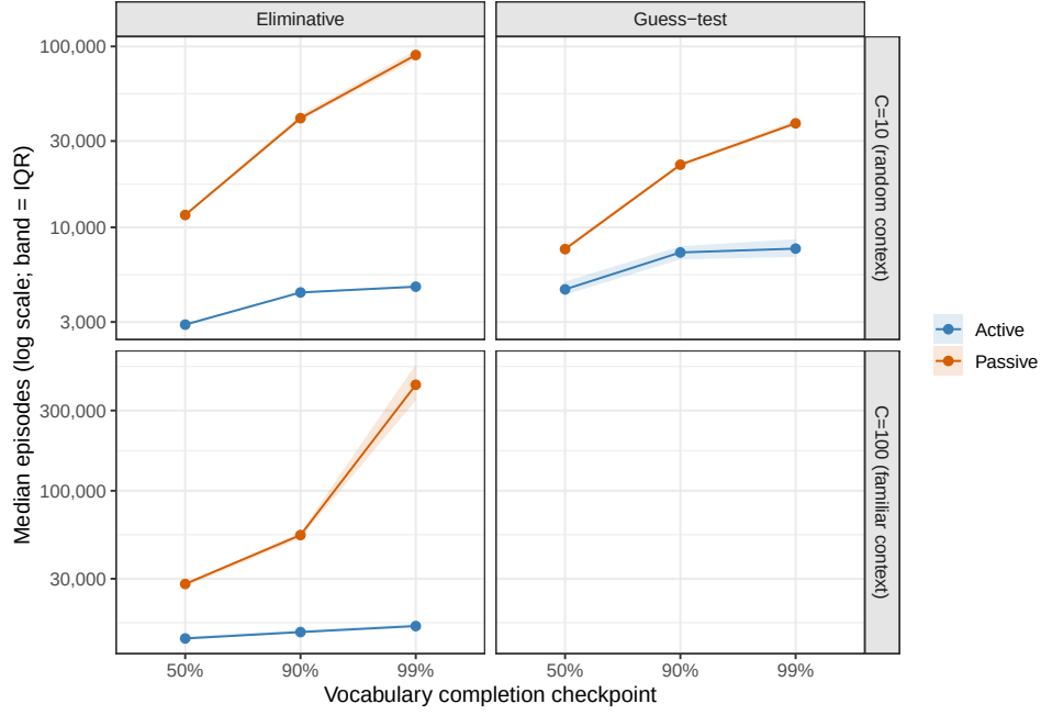
Figure 7. Median episodes (log scale; band = interquartile range) to reach 50%, 90%, and 99% of a Zipfian ( a = 1 ), M = 1000 -word vocabulary, active vs. passive target selection, by learning mechanism and context size. The C = 100 row uses familiar context selection, since no random-context run completes at C = 100 . The active/passive gap widens steadily with the completion target rather than being a fixed multiplicative constant.
