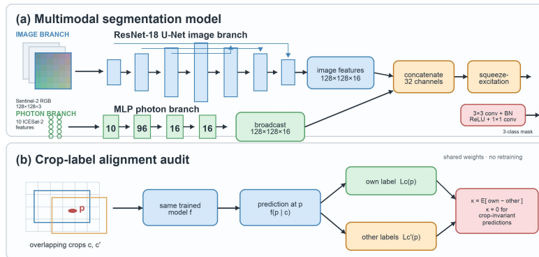
Figure 2. Model and audit schematic. The sea-ice model uses an ImageNet-initialized ResNet-18 U-Net image branch and, in photon-enabled runs, an MLP branch for ICESat-2 features. The audit keeps weights fixed and compares agreement with the current crop’s label against other crops’ labels for the same source pixel.
