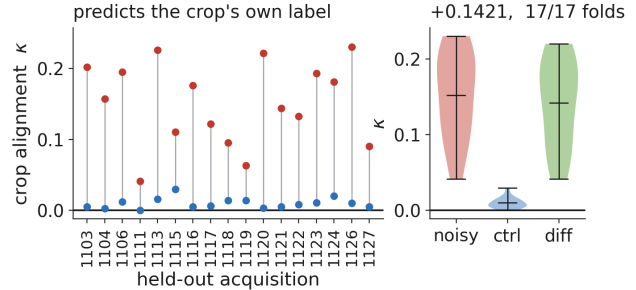
Figure 4. Optical-only primary crop-label alignment (seed 42) per held-out acquisition. Red is the model trained on crop-noisy labels, blue its matched control trained on labels regenerated once per scene. Zero is the theoretical identity for crop-invariant predictors; the trained control is empirical and need not equal it.
