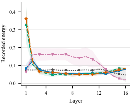
(a) Representation energy
