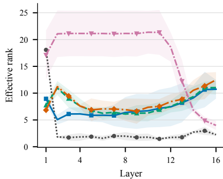
(b) Rank trajectory
