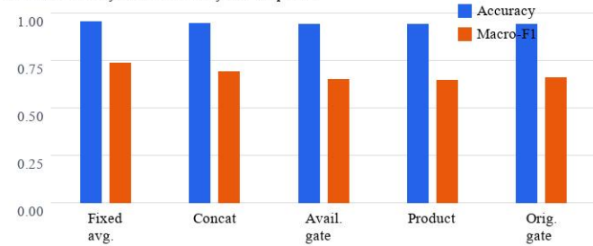
Held-out accuracy and macro-F1 by fusion operator
