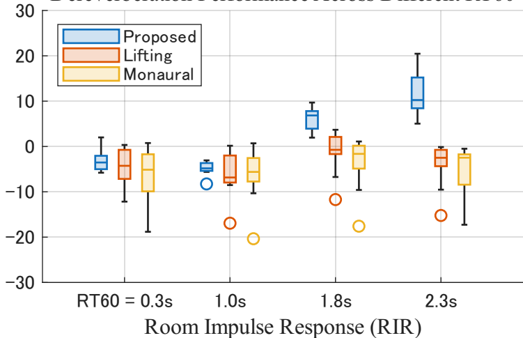
Dereverberation Performance Across Different RT60
