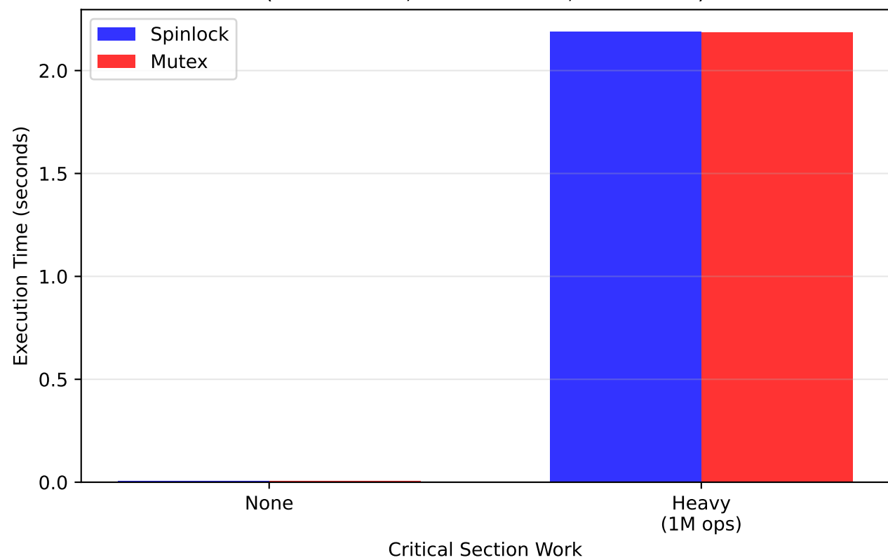
Performance vs Critical Section Length (2 Producers, 2 Consumers, Buffer=20)
