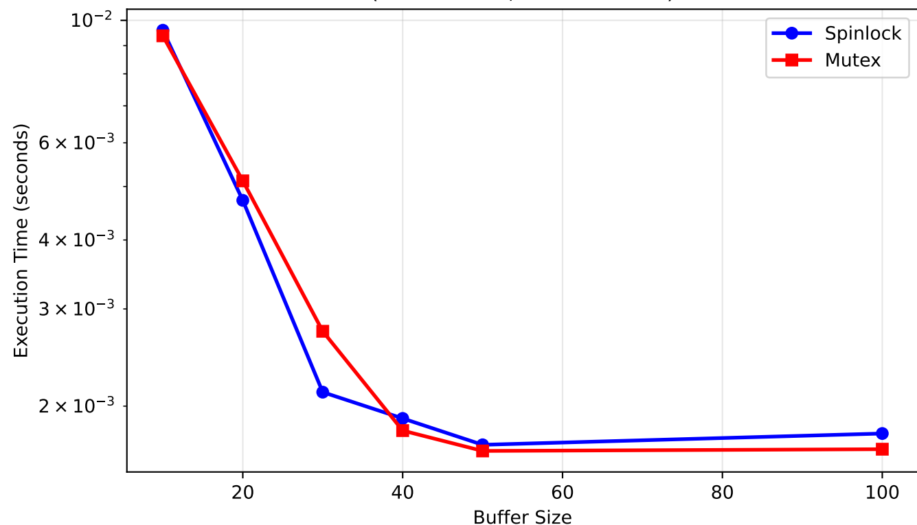
Performance vs Buffer Size (2 Producers, 2 Consumers)
