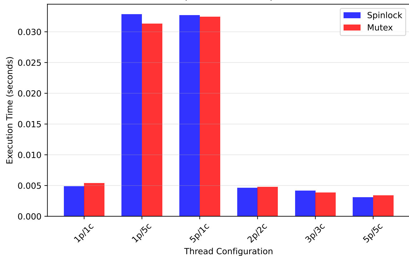
Performance vs Thread Count (Buffer Size = 20)
