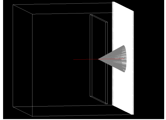
FIG. 5 Geant4 simulation of the simplified RICH detector. The particle track (red) is incident on some material with a refractive index n , called the radiator. In this case, an aerogel radiator is simulated. The resulting Cherenkov photons (gray) emitted in a cone are incident on a square array of sensitive photodetectors. In practice, the detector array is often a ring, and there are optics surrounding the device to guide photons towards the detector.
