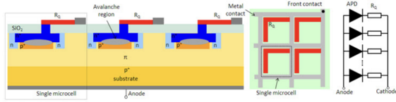
FIG. 4 Cross section of SiPM. SiPMs are externally biased such that each avalanche photodiode is at breakdown voltage, allowing for electron avalanches. The gain from a SiPM roughly matches that of a MCP-PMT at 10^5 – 10^6 times amplification 15
