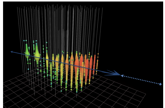
FIG. 10 IceCube event display. Multiple charged particle tracks can be distinguished. Maximum likelihood methods can be used to parse the muon tracks to identify neutrino interactions in the water 28 .
