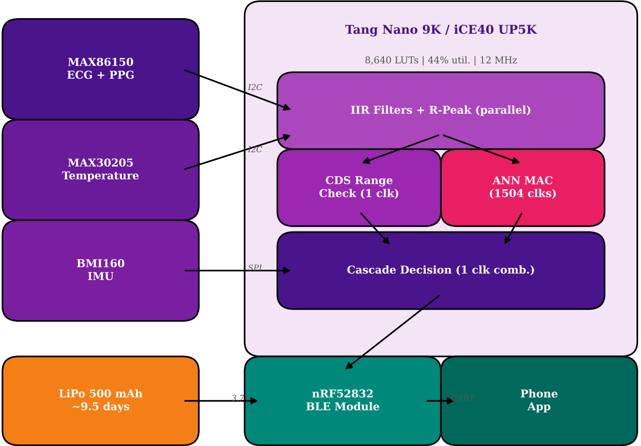
Track B: FPGA (Parallel Hardware)
